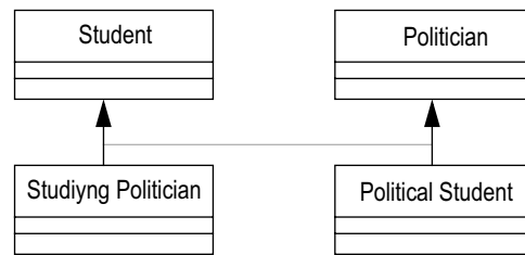
Figure 1: commonSuperType Example.
